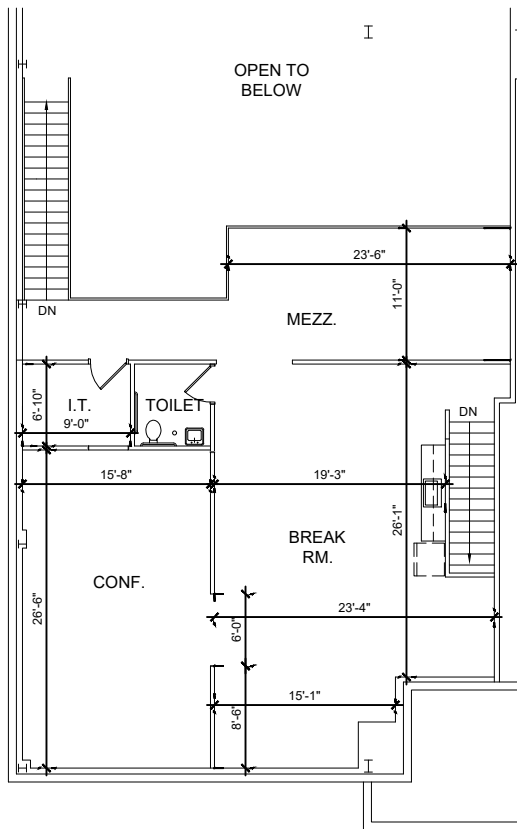
SUITE 1 - MEZZANINE PLAN
